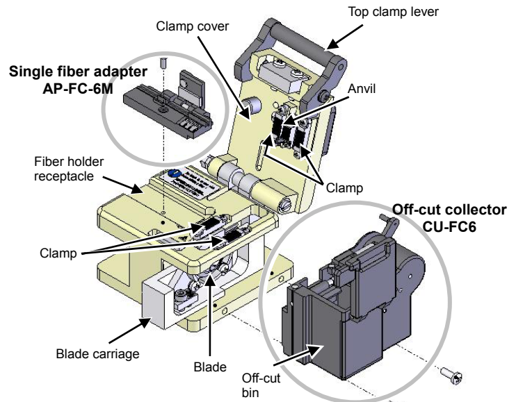
< Fiber cleaver FC-6M(-C)/6S(-C) >
